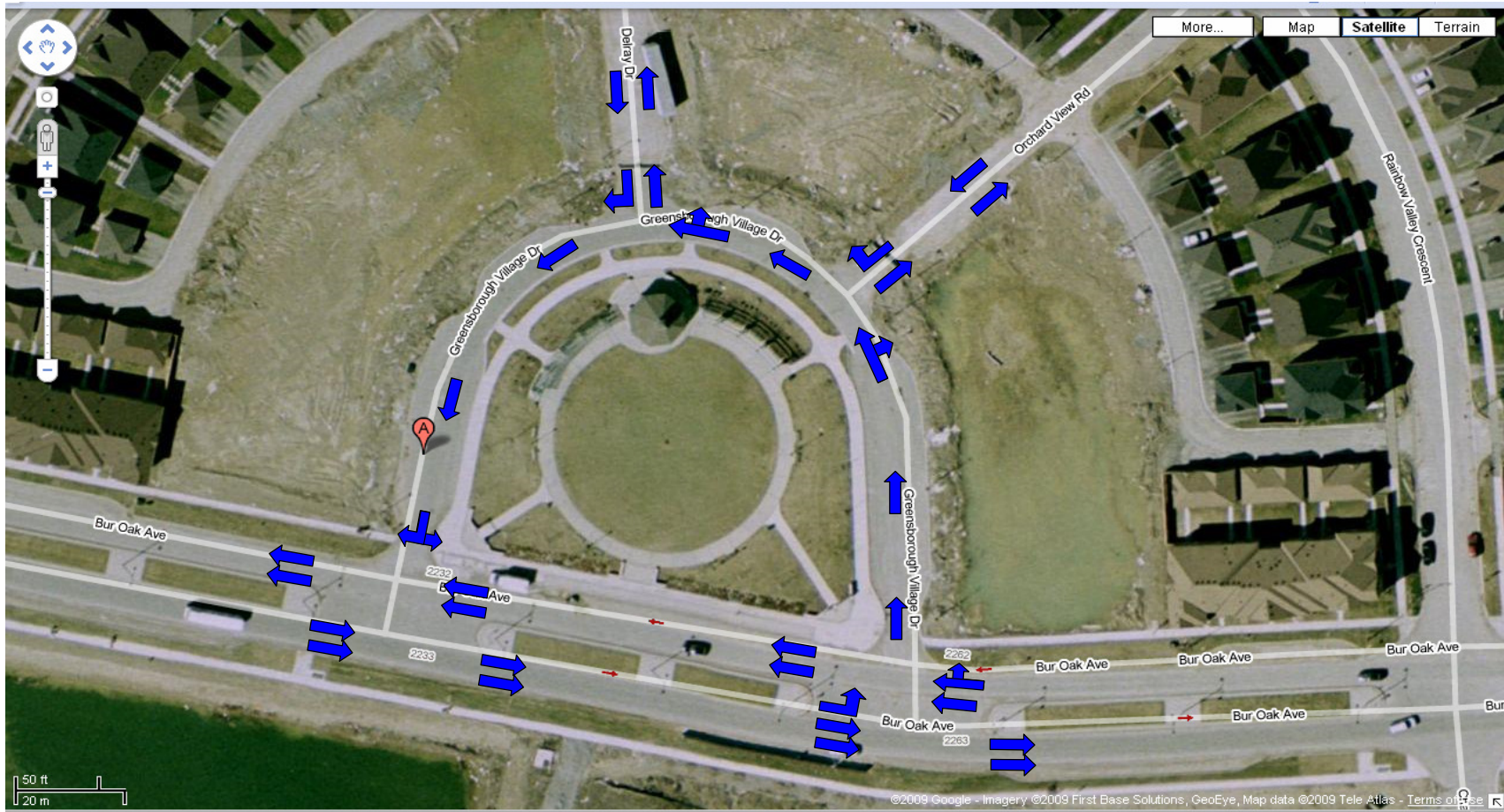
Greensborough Village Dr Oneway Concept
